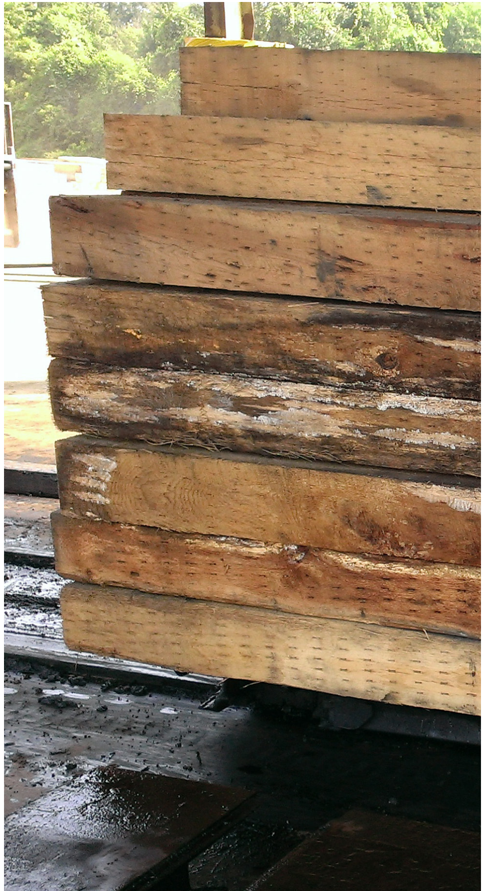
FIGURE 8. Stack burned (partially rotten) ties going into the treatment cylinder. These ties have lost some of their potential for excellent service and this loss cannot be recovered.
